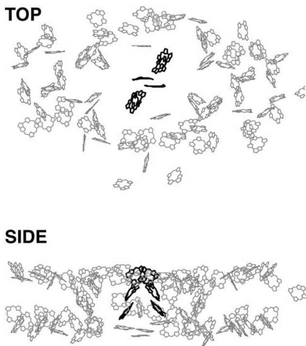
FIGURE 1 Top ( upper ) and side ( lower ) view of the spatial arrangement of chl a molecules in the PSI core of Synechococcus elongatus , as derived from the 2.5 Å structural model. The gray molecules represent the antenna chls whereas the black molecules represent the chls in the RC. For clarity the phytol tails of the molecules have been omitted.
